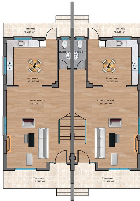
GROUND FLOOR PLAN AREA 126.00 M 2
