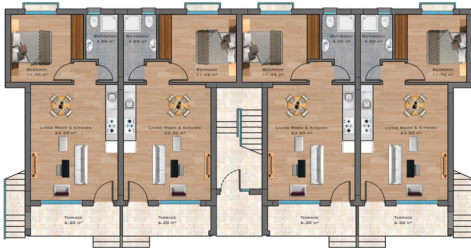
GROUND FLOOR PLAN AREA 228.00 M 2
