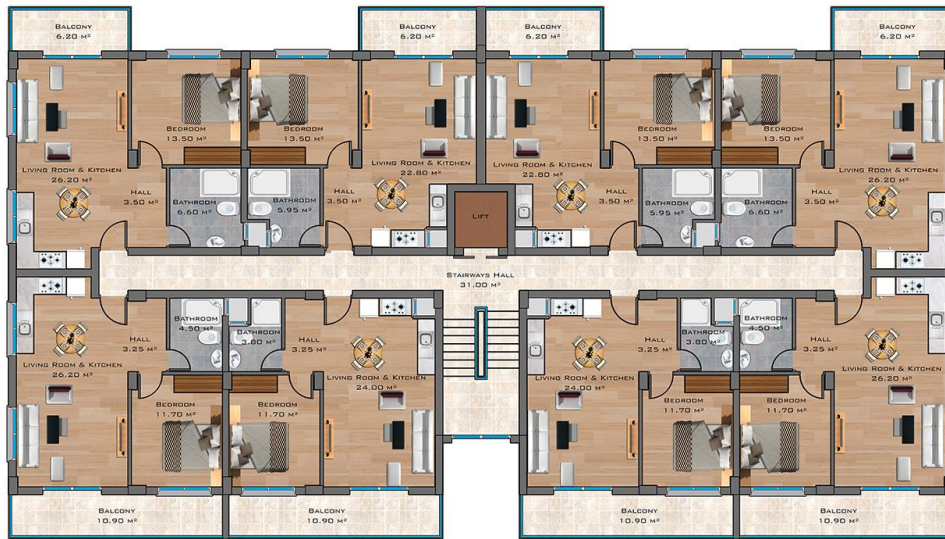
TYPE FLOOR PLAN AREA 530.00 m 2
