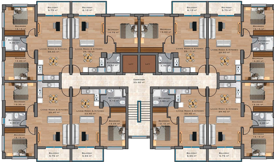
TYPE FLOOR PLAN AREA 570.00 M 2
